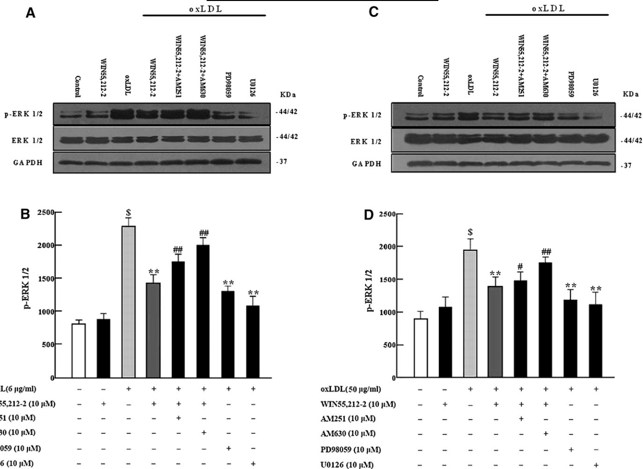
Fig. 5. Effects of the cannabinoid WIN55,212-2 on oxLDL-induced ERK1/2 activation in cultured murine macrophages. After treatment with oxLDL alone or combined with WIN55,212-2 (10 µM), AM251 (10 µM), AM630 (10 µM), PD98059 (10 µM), or U0126 (10 µM) for 10 min, 20 µg of protein was prepared and p-ERK1/2 was detected by Western blot analysis with anti-phospho-ERK1/2. Incubation with oxLDL significantly increased ERK1/2 activation compared with vehicle control ( $ P < 0.01). ERK1/2 activation was inhibited by coinubation with WIN55,212-2, PD98059, or U0126 compared with vehicle control ( ** P < 0.01); effects of WIN55,212-2 were markedly attenuated by AM251 or AM630 ( # P < 0.05; ## P < 0.01). Data are expressed as relative optical density compared with GAPDH from three separate experiments with duplicate samples. A and B: RAW264.7 macrophages. C and D: primary peritoneal macrophages. AM251, N-(piperidin-1-yl)-5-(4-iodophenyl)-1-(2,4-dichlorophenyl)-4-methyl-1H-pyrazole-3-carboxamide; AM630, 6-iodo-2-methyl-1-[2-(4-morpholinyl)ethyl]-1H-indol-3-yl] (4-methoxyphenyl) methanone; GAPDH, glyceraldehyde phosphate dehydrogenase; oxLDL, oxidized low-density lipoprotein; PD98059, 2-(2-amino-3-methoxyphenyl)-4H-1-benzopyran-4-one; ROS, reactive oxygen species; U0126, 1,4-diamino-2,3-dicyano-1,4-bis(o-aminophenylmercapto) butadiene monoethanolate; WIN55,212-2, (R)-(+)-2,3-dihydro-5-methyl-3-(4-morpholinylmethyl) pyrrolo[1,2,3-de]-1,4-benzoxazin-6-yl]-1-naphthalenylmeth anone mesylate.
