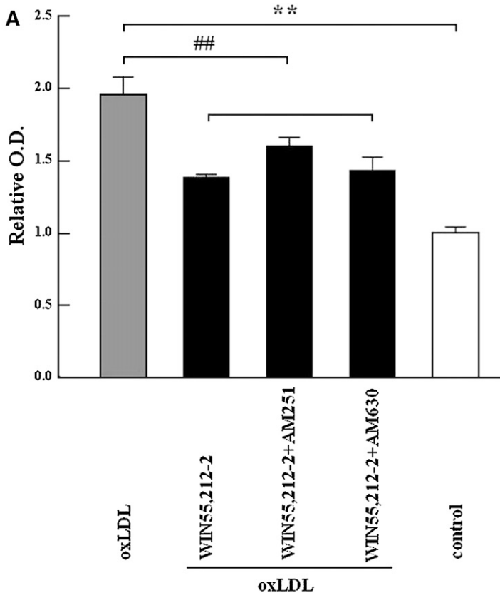
Fig. 4. Effects of the cannabinoid WIN55,212-2 on oxLDL-induced NF-kappa B DNA-binding activity in RAW264.7 macrophages. After treatment with oxLDL (6 \mu\text{g}/\text{ml} ) alone or in combination with WIN55,212-2 (10 \mu\text{M} ) and AM251 (5 \mu\text{M} ) or AM630 (5 \mu\text{M} ) for 24 h, 8 \mu\text{g} of nuclear extract was prepared and subjected to EMSA analysis. Data in Fig. 4A are expressed as mean \pm SEM of the relative optical density from three separate experiments with duplicate samples. In Fig. 4B , the upper bands reflect NF-kappa B bound to DNA and the lower bands show nonspecific probe. **P < 0.01 compared with vehicle (DMEM) control (represented by a white bar); ##P < 0.01 compared with oxLDL treatment (represented by a gray bar). AM251, N-(piperidin-1-yl)-5-(4-iodophenyl)-1-(2,4-dichlorophenyl)-4-methyl-1H-pyrazole-3-carboxamide; AM630, 6-iodo-2-methyl-1-[2-(4-morpholinyl)ethyl]-1H-indol-3-yl] (4-methoxyphenyl) methanone; oxLDL, oxidized low-density lipoprotein; WIN55,212-2, (R)-(+)-2,3-dihydro-5-methyl-3-(4-morpholinylmethyl) pyrrolo[1,2,3-de]-1,4-benzoxazin-6-yl]-1-naphthalenylmeth anone mesylate.
